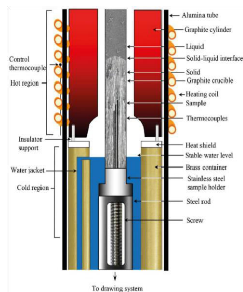
Fig. 1: Bridgman furnace scheme (Douglas, 2020).
