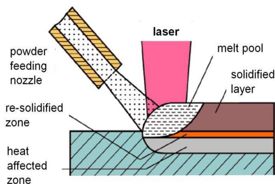
Fig. 3: Schematic of direct metal deposition.
