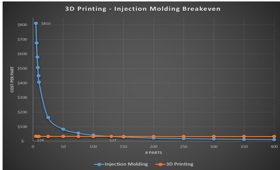
Fig. 2: Cost analysis of 3D printing vs injection moulding.
